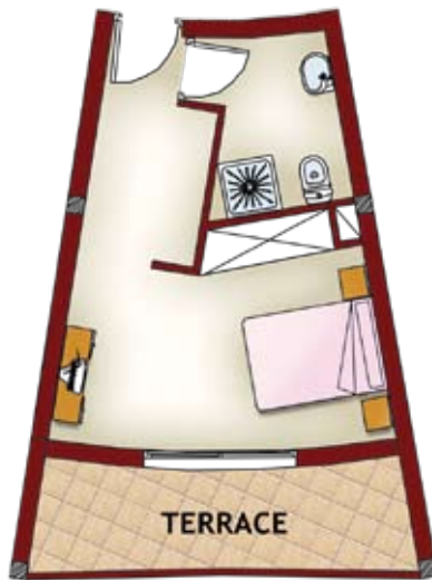
CABO DREAM APARTMENT HOTEL 1 ST , 2 ND , 3 RD AND 4 TH FLOOR CORNER MODEL
